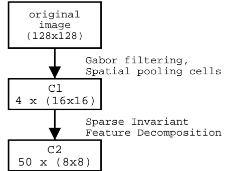
Figure 2: Wersing and Korner's hierarchy
